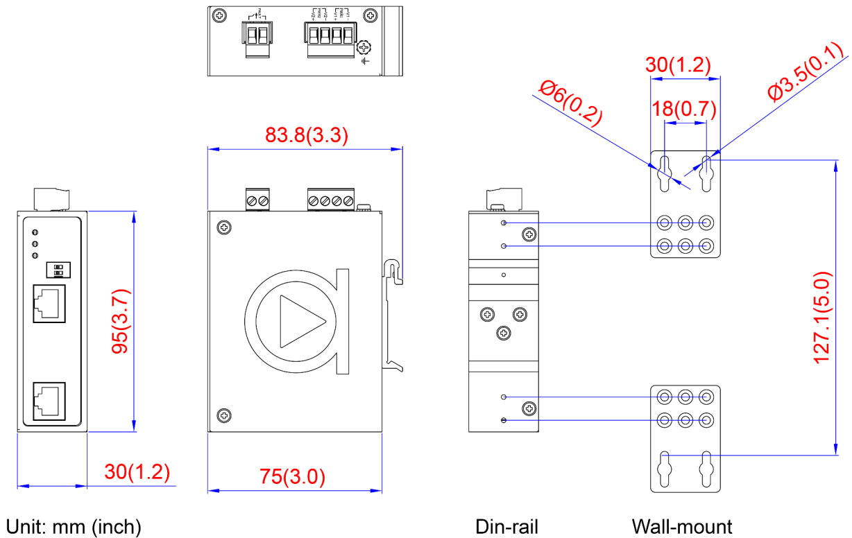
Figure 2.1 - Physical Dimensions
