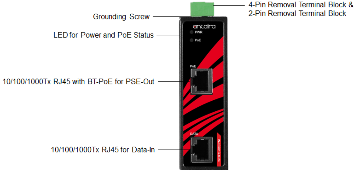
Figure 2.2 - Front View Panel
