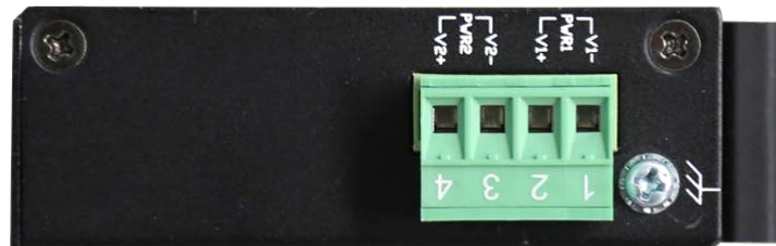
Power Inputs
