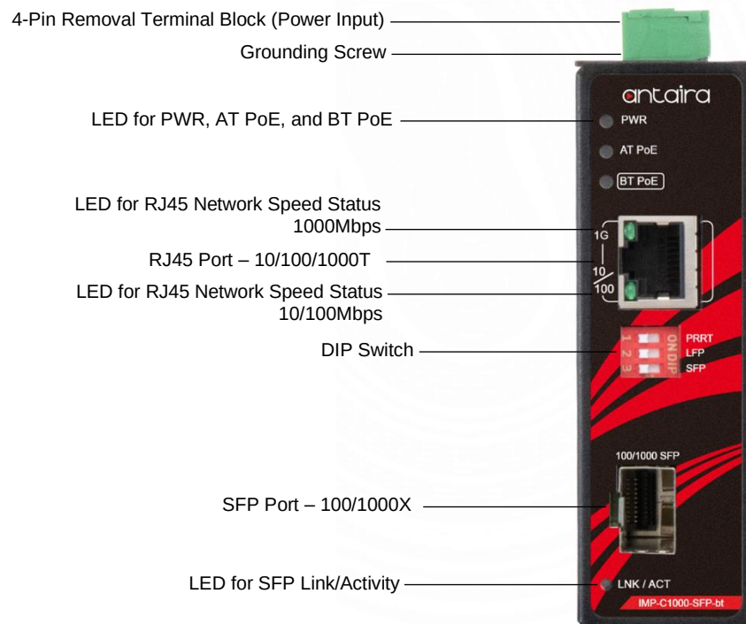
Figure 2.2 Front Panel
